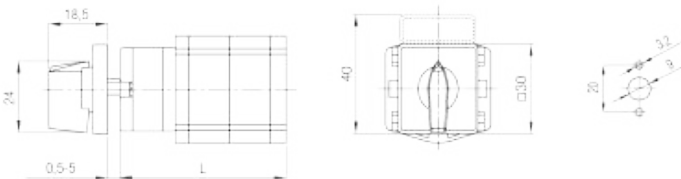
GF20R Ugradna sklopka / Front mounting (A)
