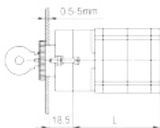
Centralna ugradnja - 10/12 Central mounting - 10/12
