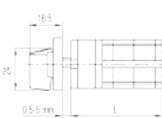
GF10 Ugradna sklopka / Front mounting (A)
