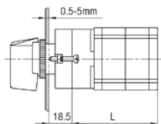
Centralna ugradnja - 09/11 Central mounting - 09/11
