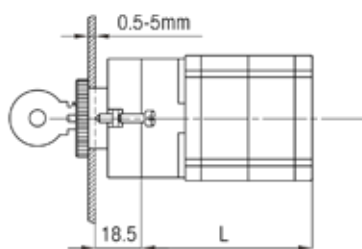
Centralna ugradnja - 10/12 Central mounting - 10/12
