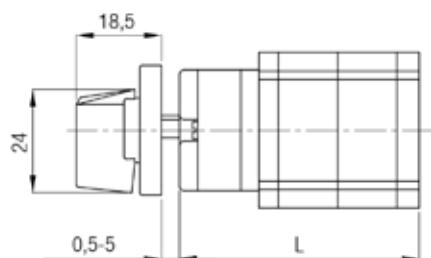
GF20R Ugradna sklopka / Front mounting (U)
