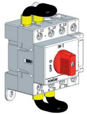
CSP80-31-40048D
